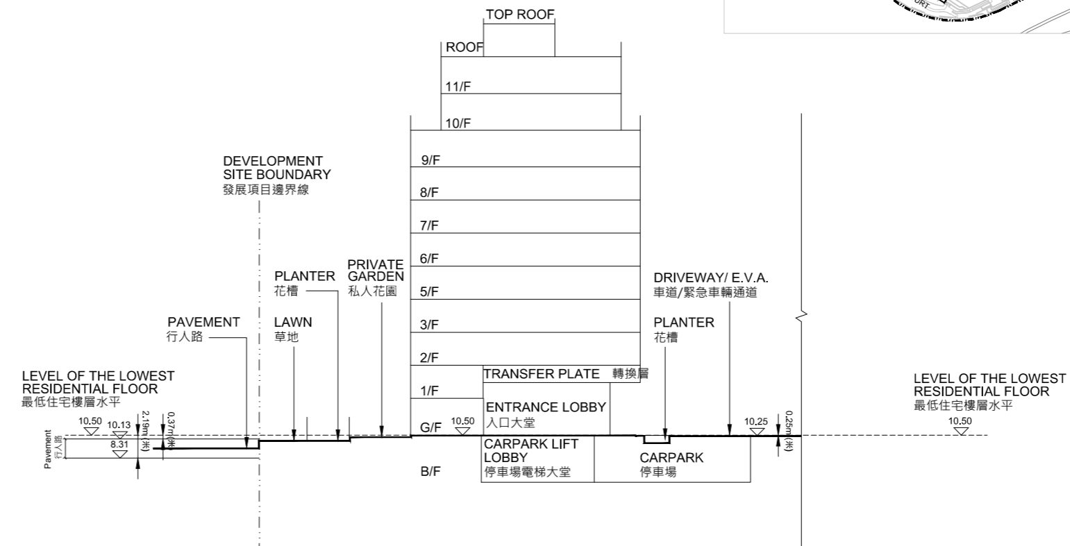
Cross-Section Plan B 橫截面圖B
