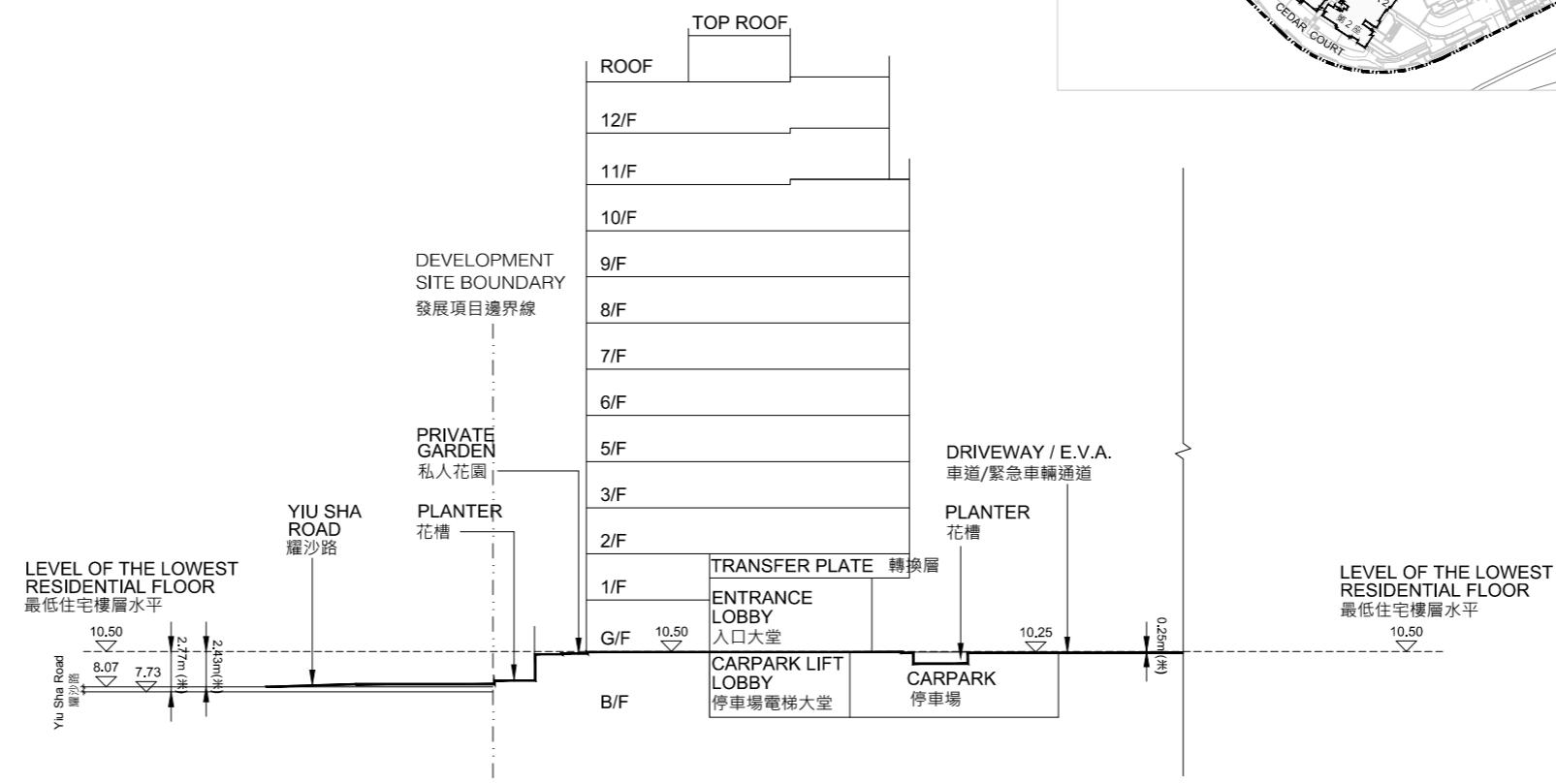
Cross-Section Plan F 橫截面圖F
