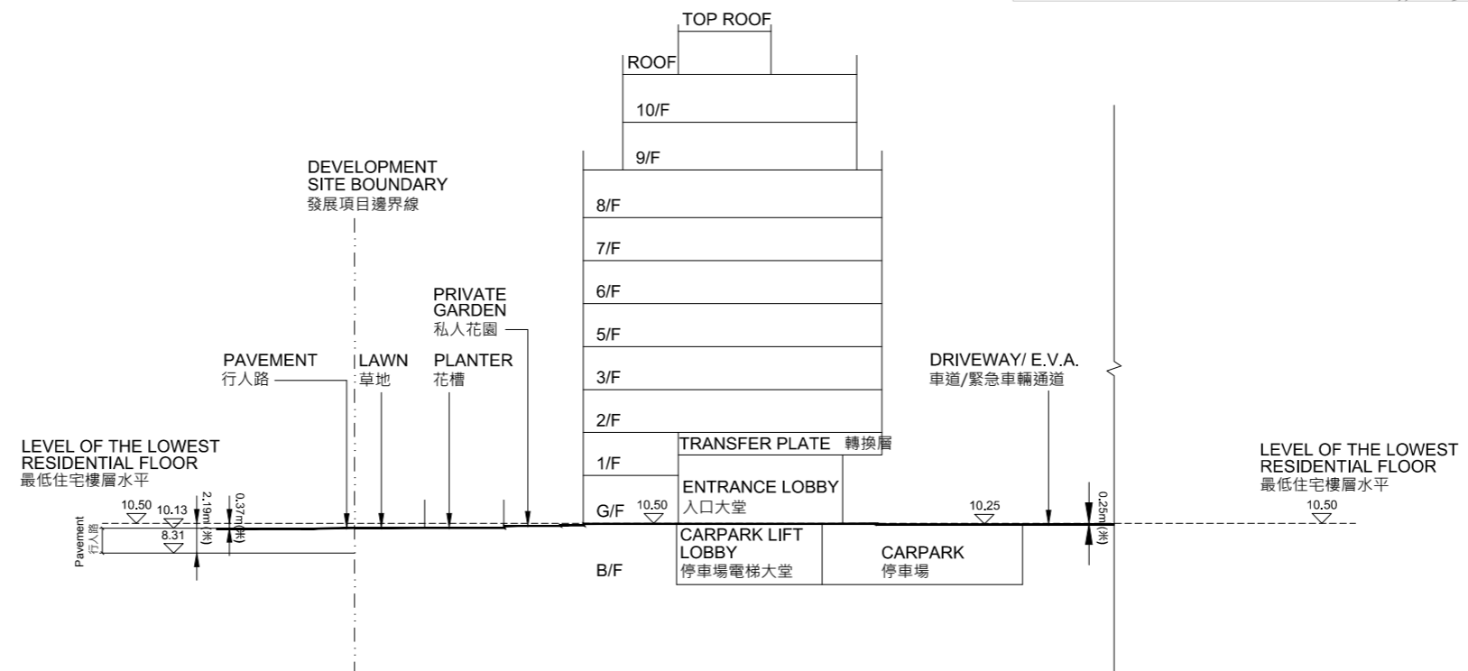
Cross-Section Plan A 橫截面圖A
