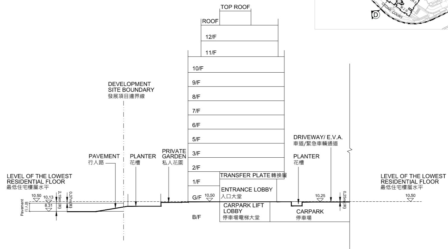
Cross-Section Plan D 橫截面圖D
