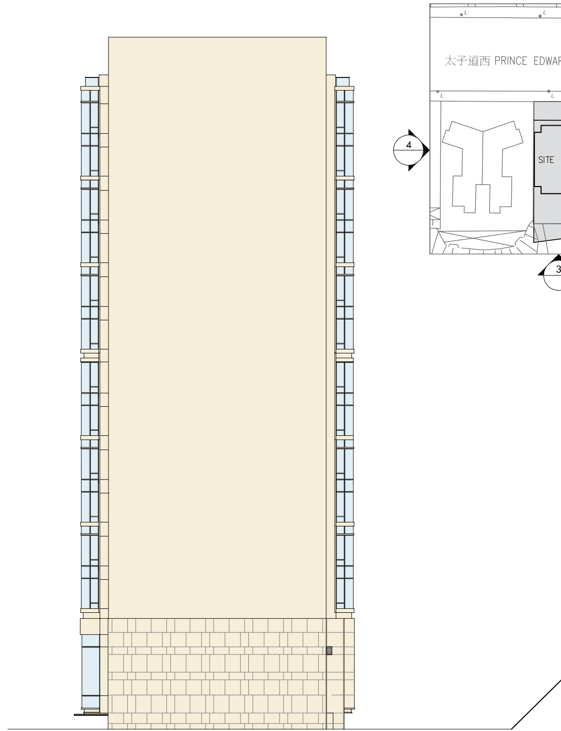
South-West Elevation 西南立面圖
