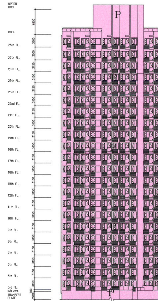
ELEVATION 6 PLAN
