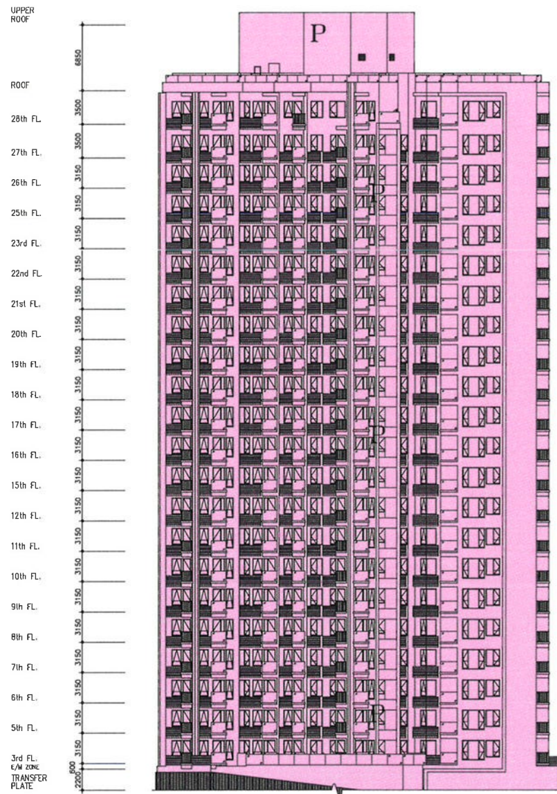
ELEVATION 4 PLAN
