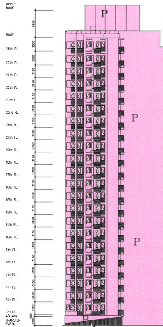
ELEVATION 5 PLAN
