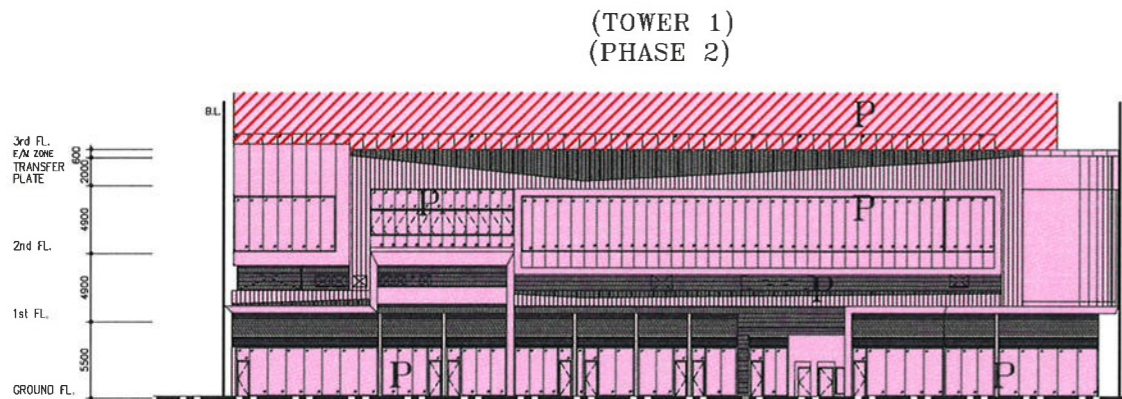
ELEVATION 9 PLAN
