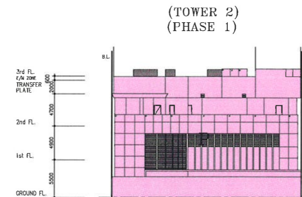
ELEVATION 10 PLAN
