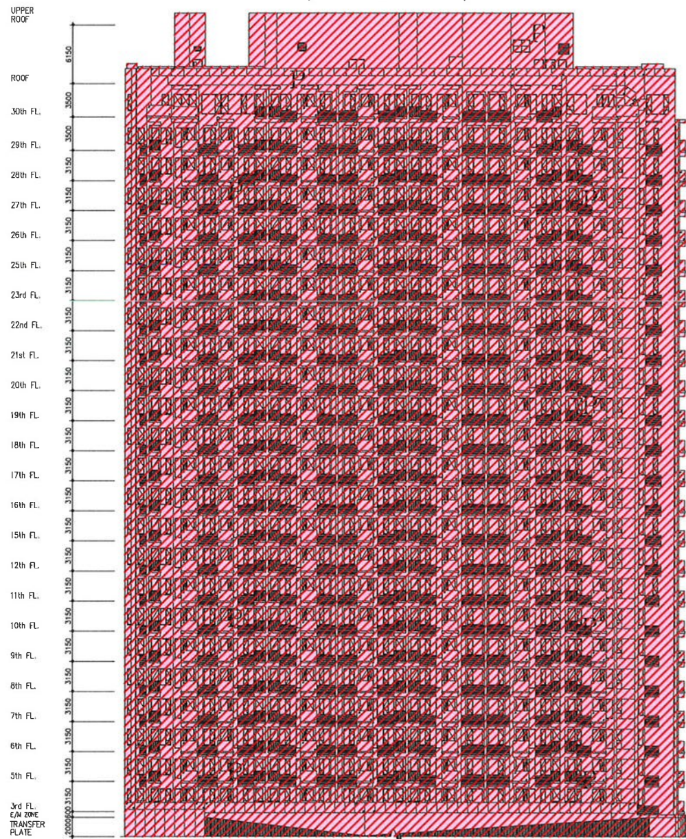
(TOWER 1) (PHASE 2)
