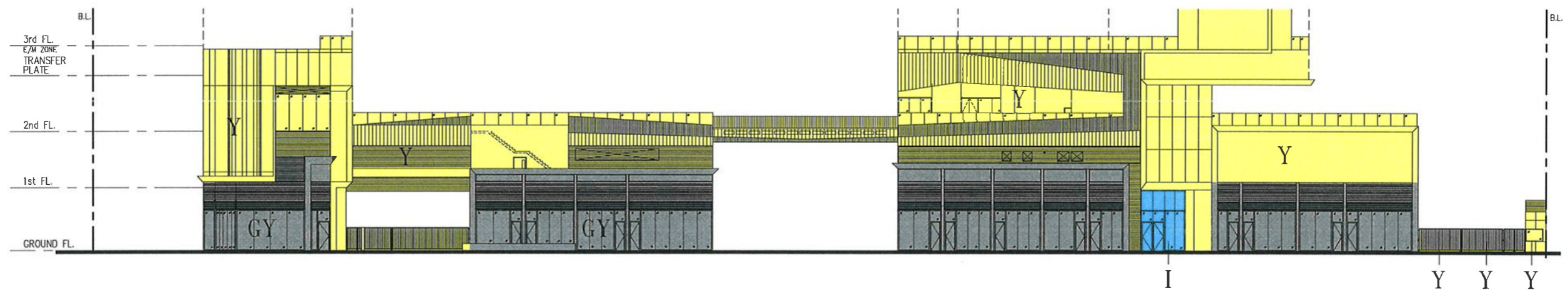
ELEVATION (FACING HANG FU STREET)
