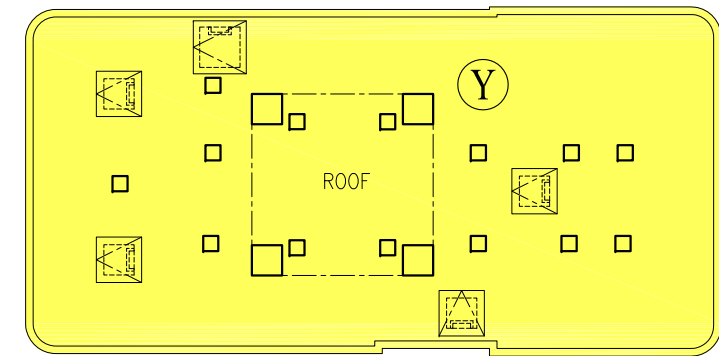
TOP ROOF PLAN
