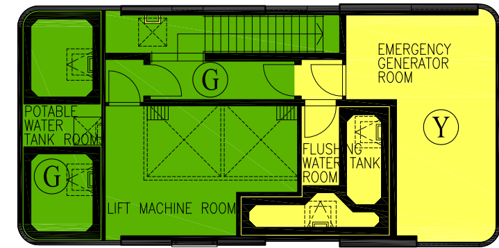
UPPER ROOF PLAN
