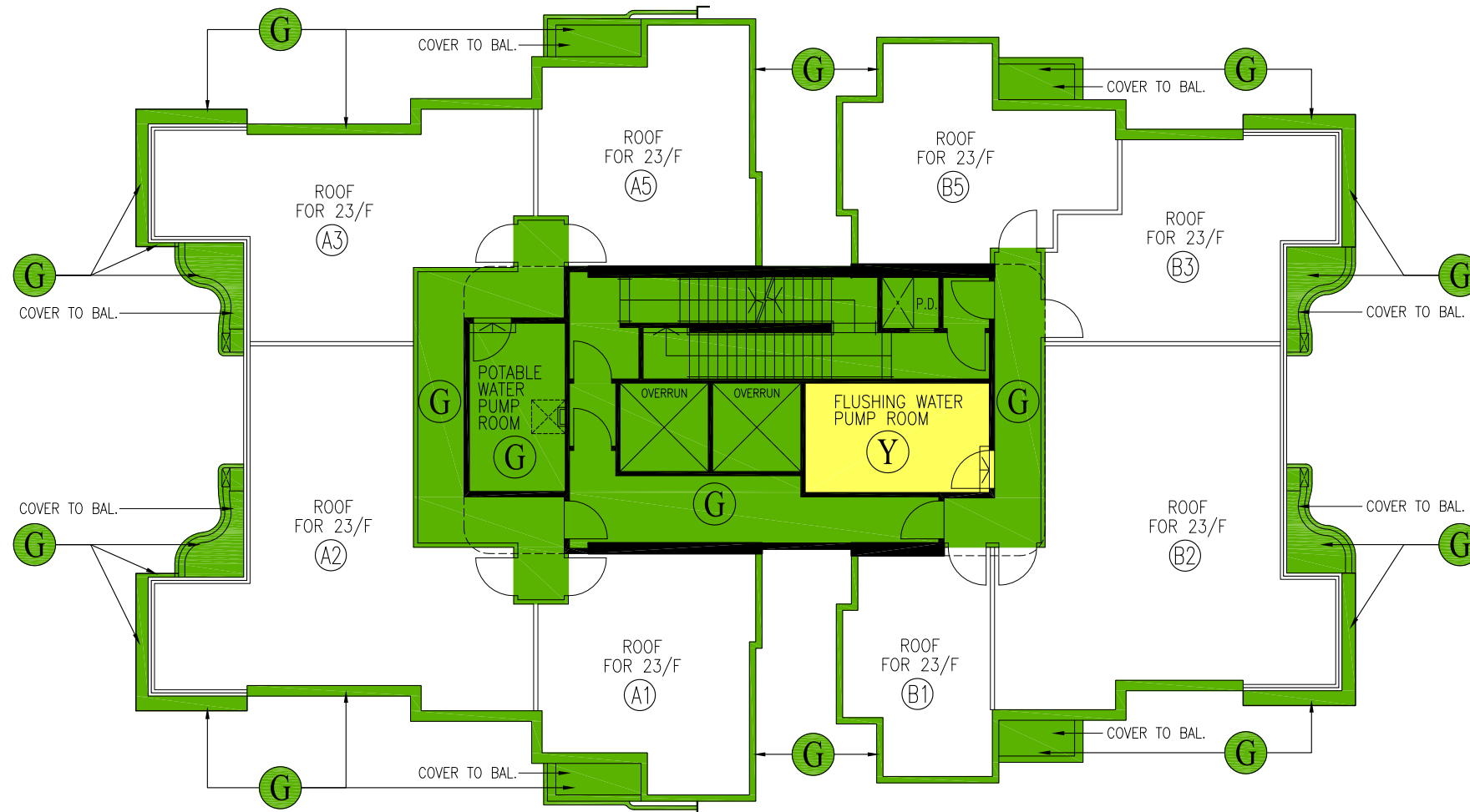
ROOF PLAN
