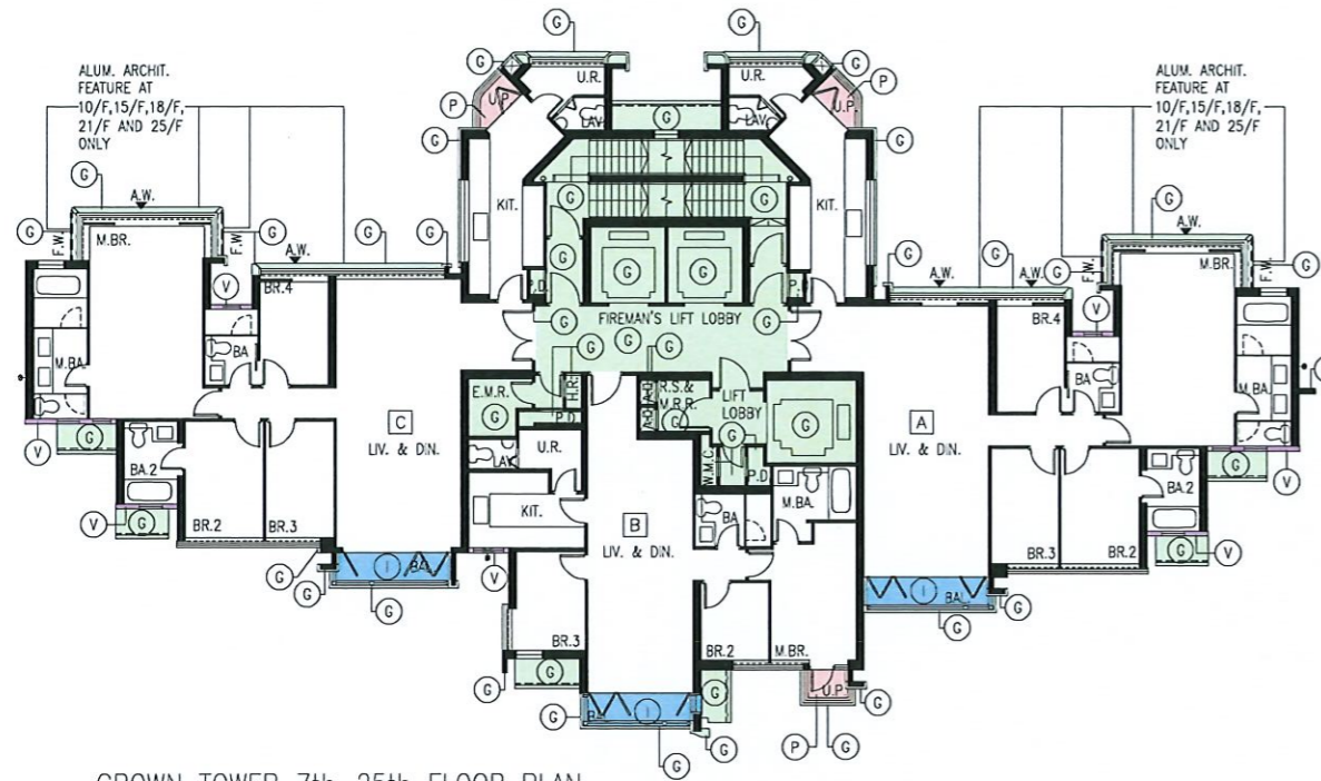
CROWN TOWER 7th-25th FLOOR PLAN
