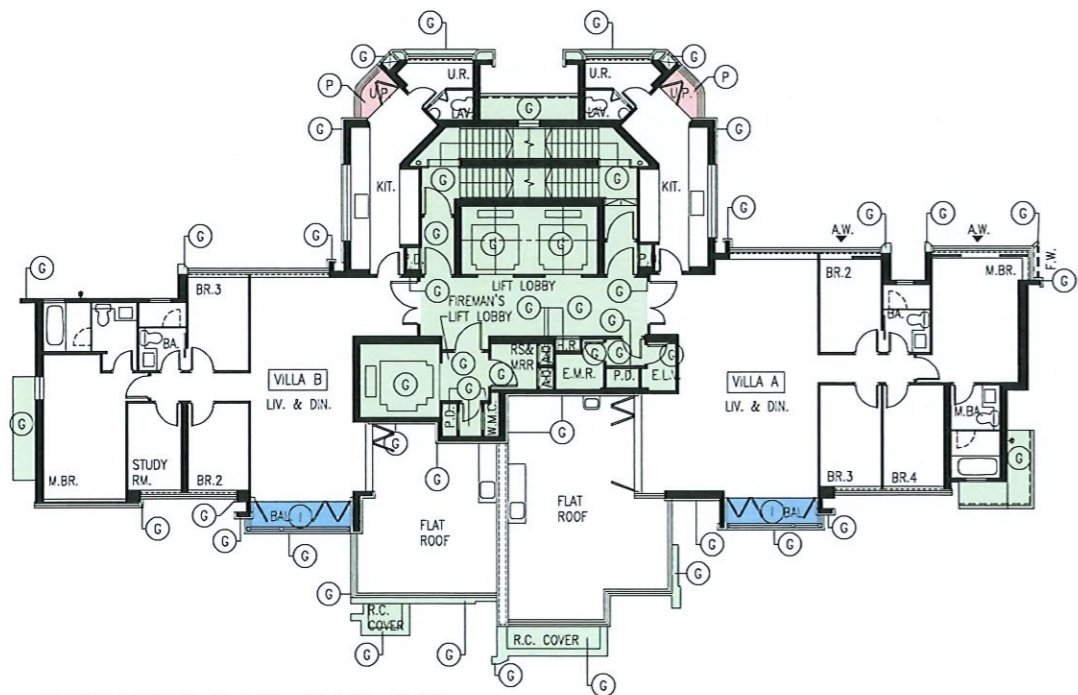
QUEEN TOWER 1 26th FLOOR PLAN
