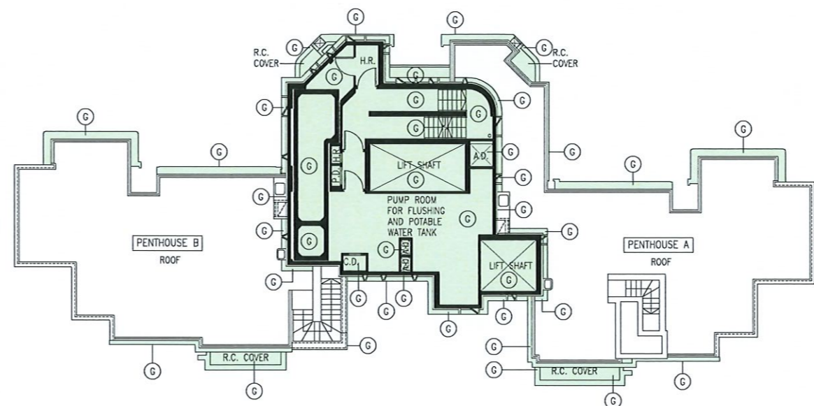
CROWN TOWER ROOF PLAN
