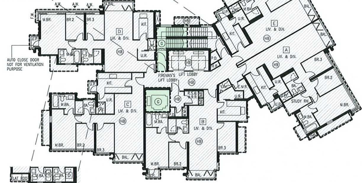
KING TOWER 2 7th-25th FLOOR PLAN
