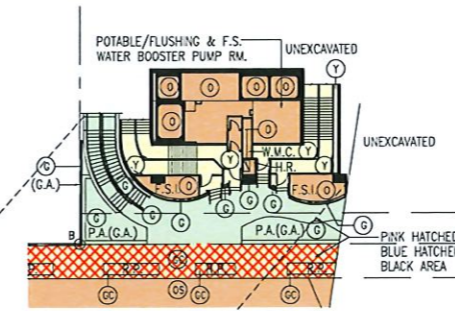
PART PLAN AT LEVEL 25.87
