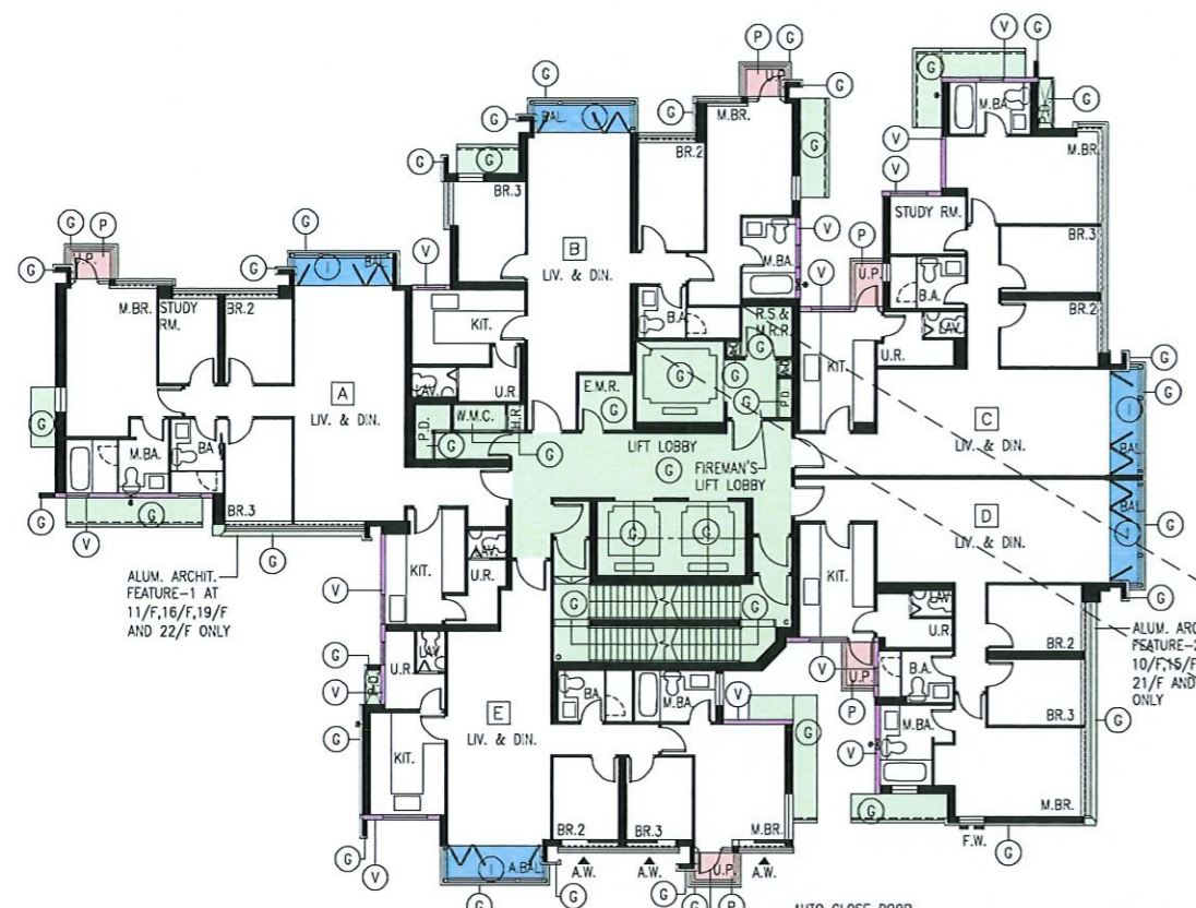
QUEEN TOWER 2 7th-25th FLOOR PLAN
