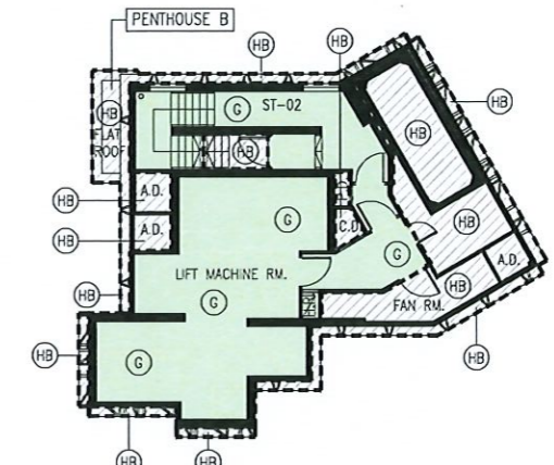
KING TOWER 2 PLANT ROOM PLAN
