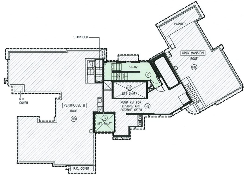
KING TOWER 2 ROOF PLAN
