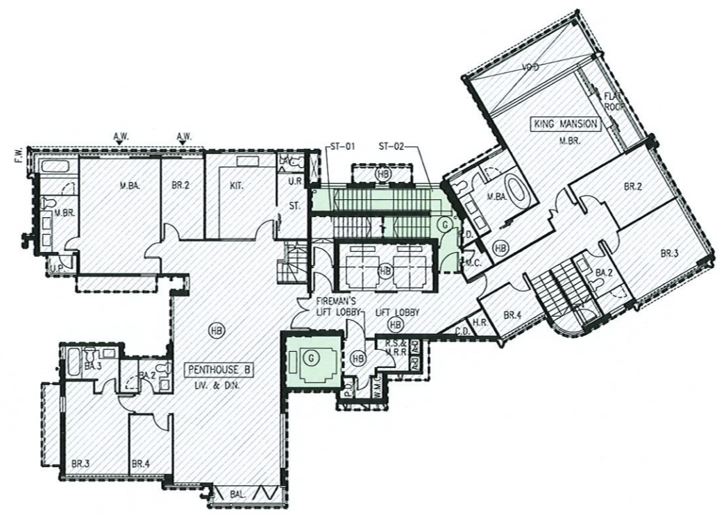
KING TOWER 2 27th FLOOR PLAN
