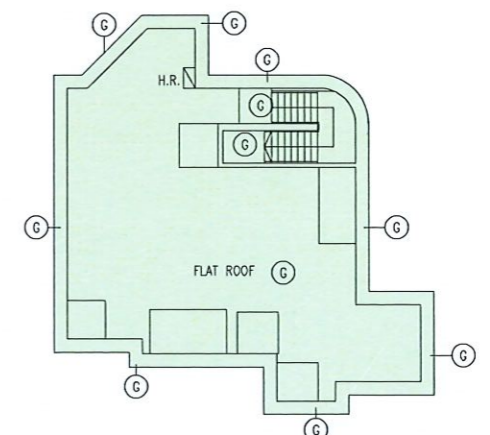
CROWN TOWER UPPER ROOF PLAN
