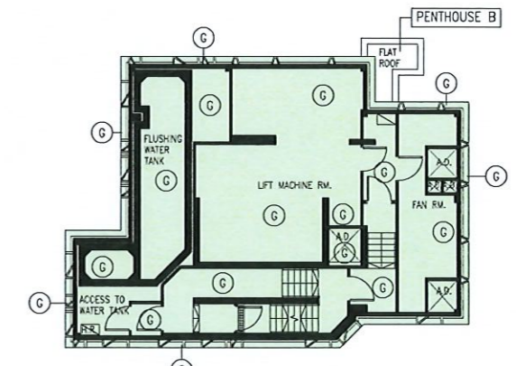
QUEEN TOWER 2 PLANT ROOM PLAN
