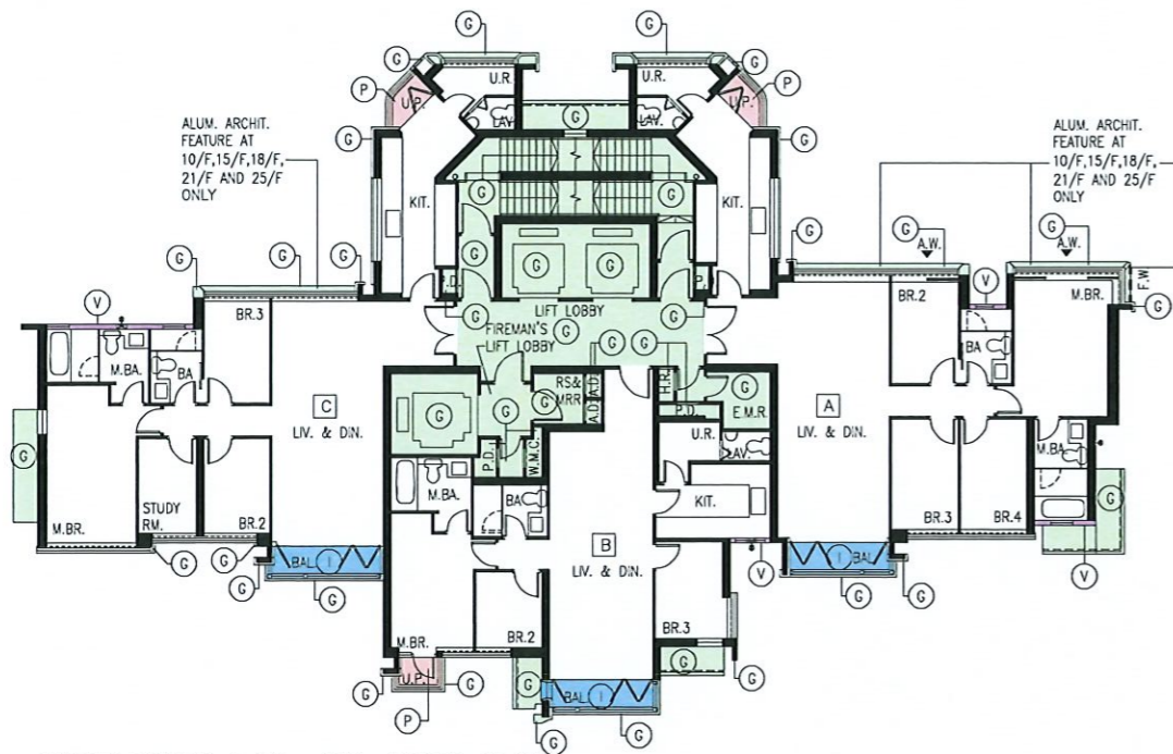
QUEEN TOWER 1 7th-25th FLOOR PLAN
