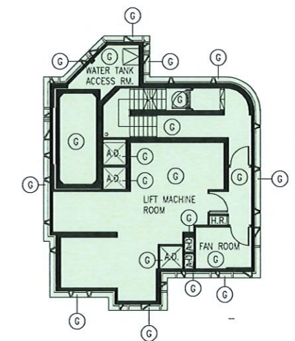
QUEEN TOWER 1 PLANT ROOM PLAN
