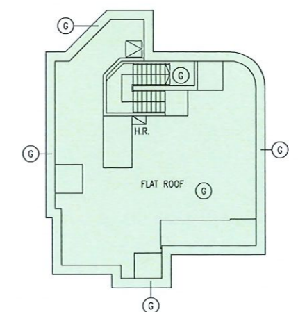
QUEEN TOWER 1 UPPER ROOF PLAN
