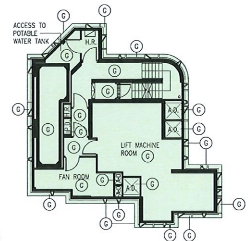
CROWN TOWER PLANT ROOM PLAN
