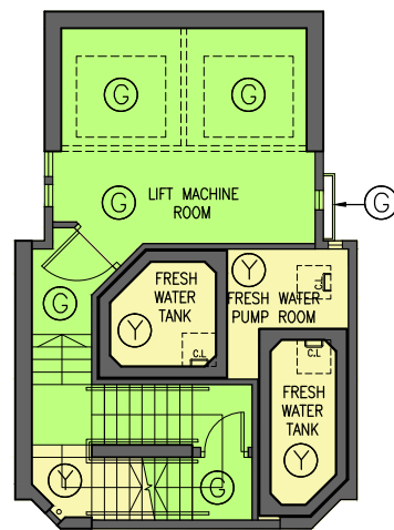
PLAN OF MACHINE ROOM
