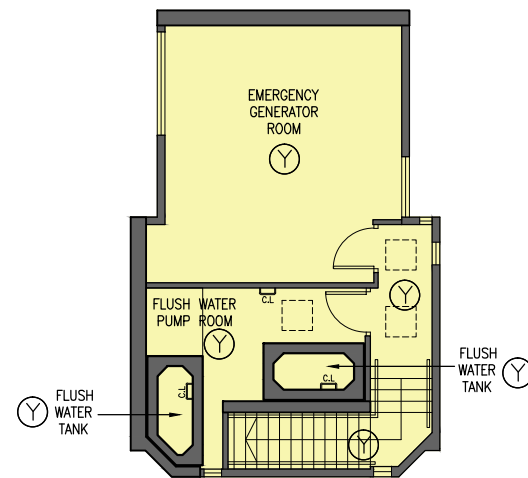
PLAN OF PUMP ROOM
